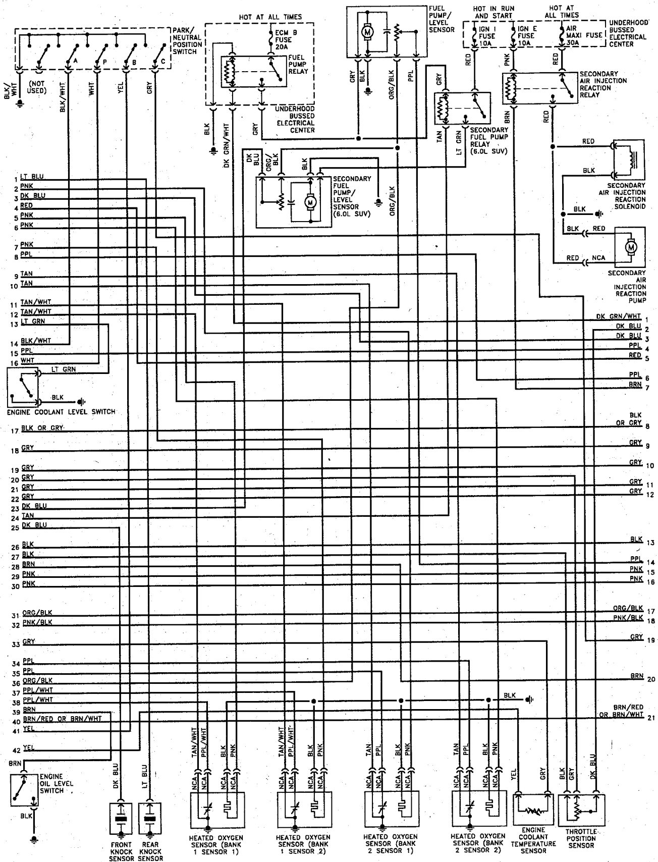
Engine control system – typical V8 (part 2 of 4, without Electronic Throttle Control)
